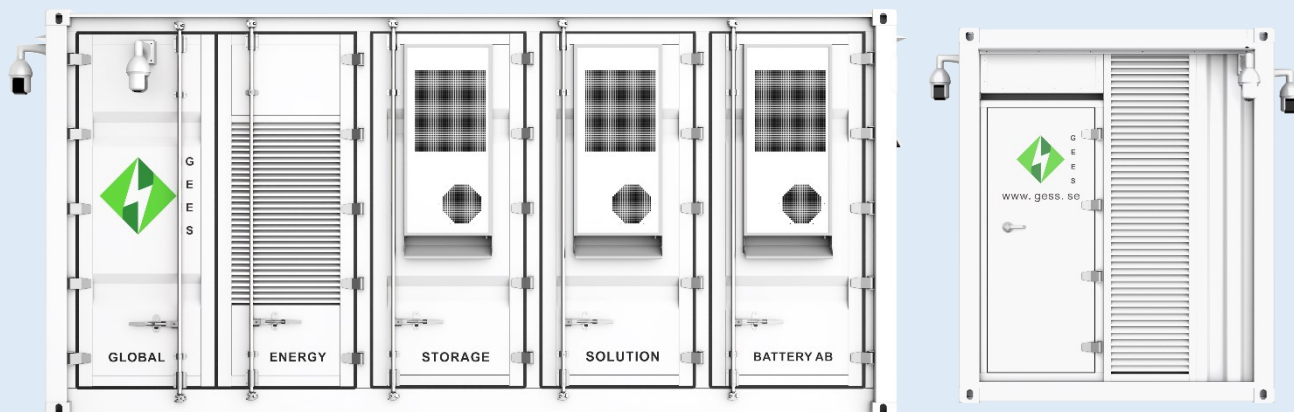
GESS-SW-1253TH-PO side views
